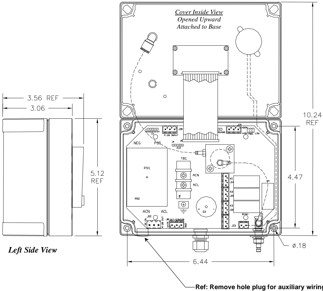
Figure 3: Mounting CO-GUARD
