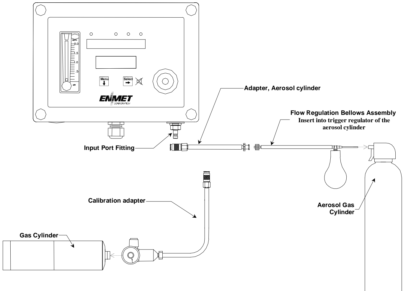
Figure 7: Calibration Adapter
