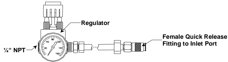
Figure 1a: Optional REGULATOR AND SAMPLE AIR HOSE
