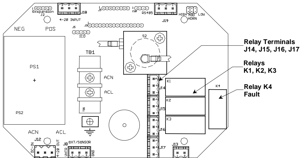
Figure 5: Relay Terminal Connections CO-GUARD
